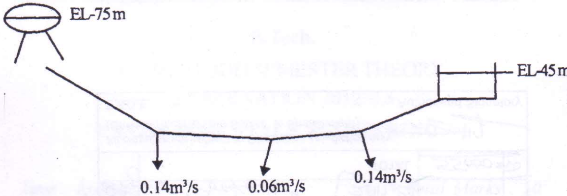
Figure 1 : Pseudo loop system
